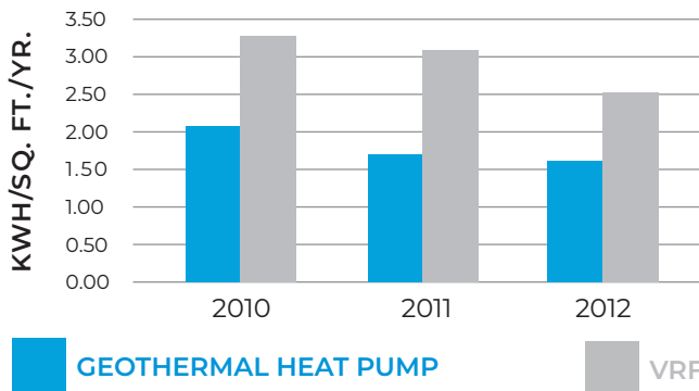
GEOHERMAL HEAT PUMP vs. VRF
