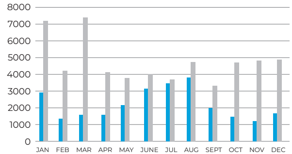
GEOHERMAL HEAT PUMP vs. VRF 2011 SYSTEM POWER (kWh)
