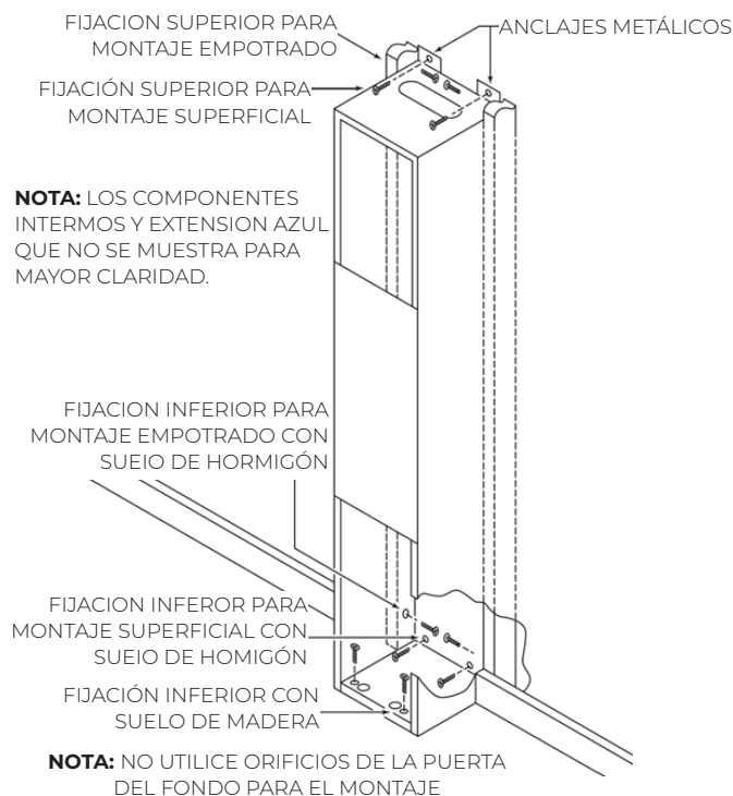
FIGURE 21 - FURNACE MOUNTING
