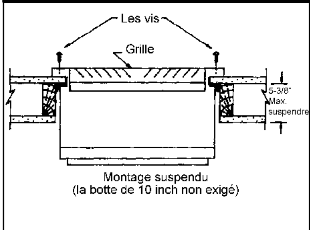
FIGURE 9 – Montage suspendu
