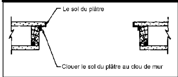
FIGURE 9 – Montage suspendu
