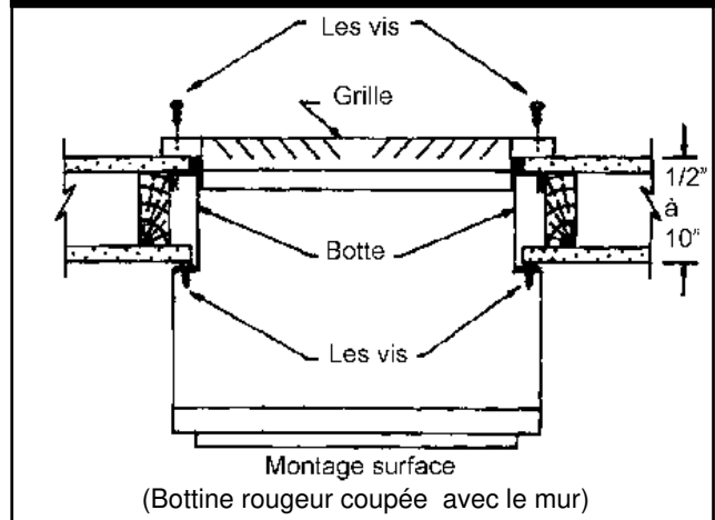
FIGURE 10 – Montage surface
