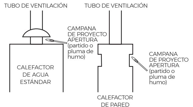
FIGURE 2 - DERAME DEL EXTRACTOR
