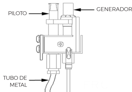
FIGURA 22 - PILOT AND GENERATOR
