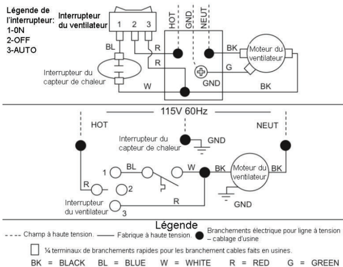
FIGURE F - CABLAGE
