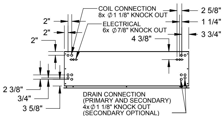
REAR VIEW (COIL CONNECTION)
