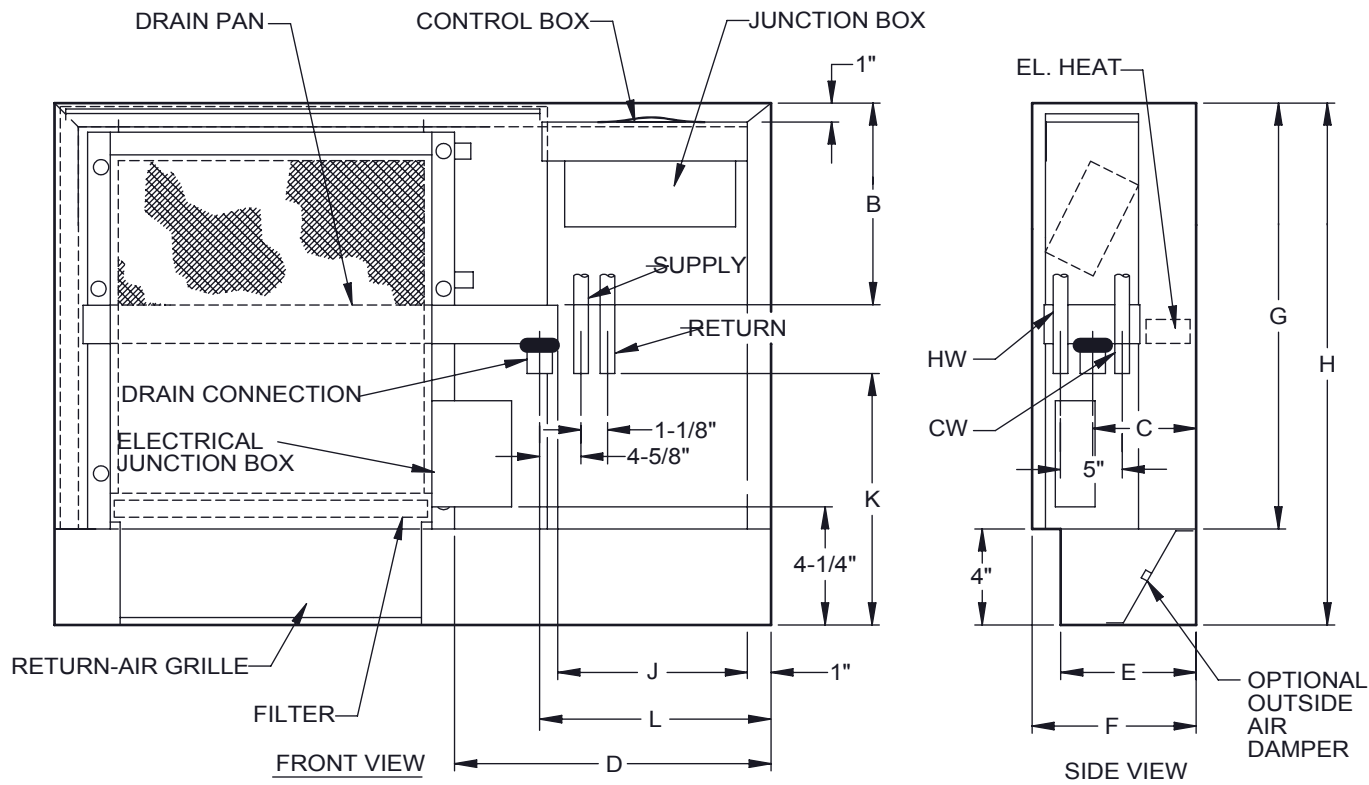
10" HANDED SIDE CABINET EXTENSION WITH EXTENDED DRAIN PAN
