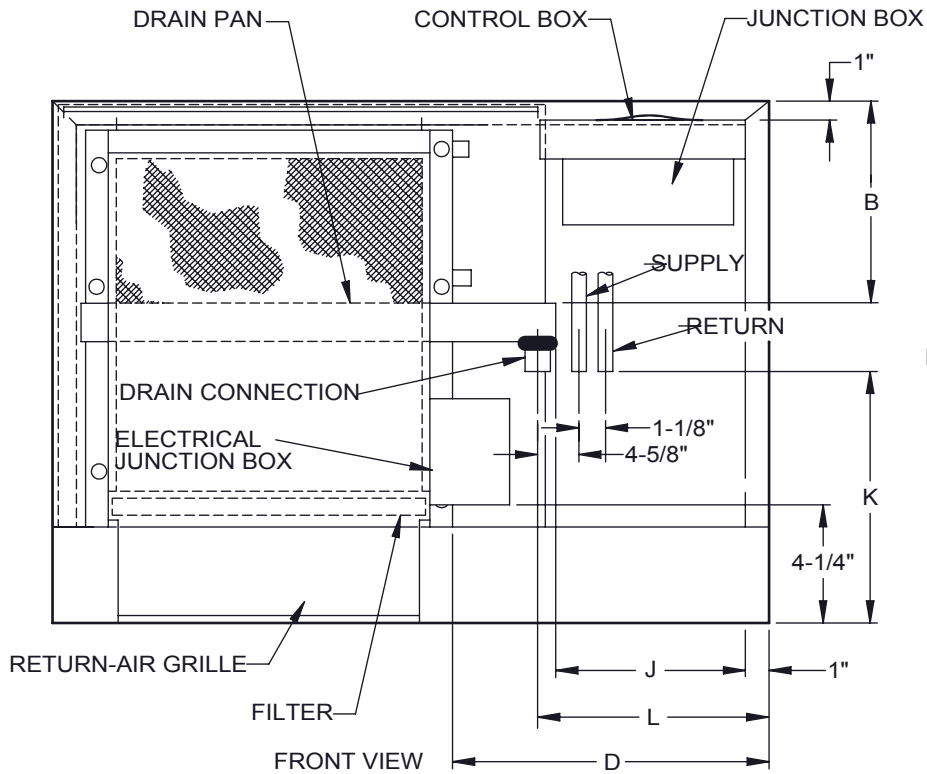
8" HANDED & 8" CABINET EXTENSION & EXTENDED DRAIN PAN
