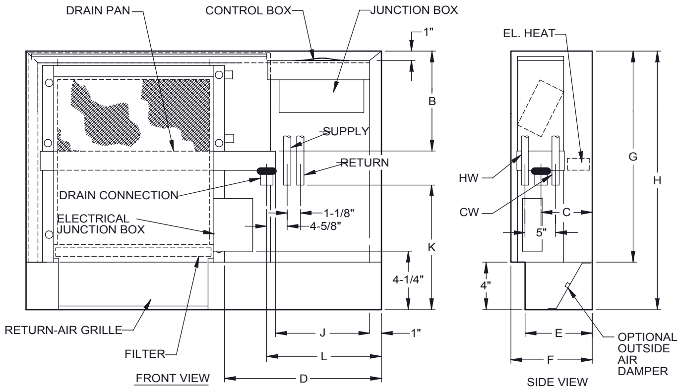
10" HANDED & 10" OPPOSITE CABINET EXTENSION & EXTENDED DRAIN PAN
