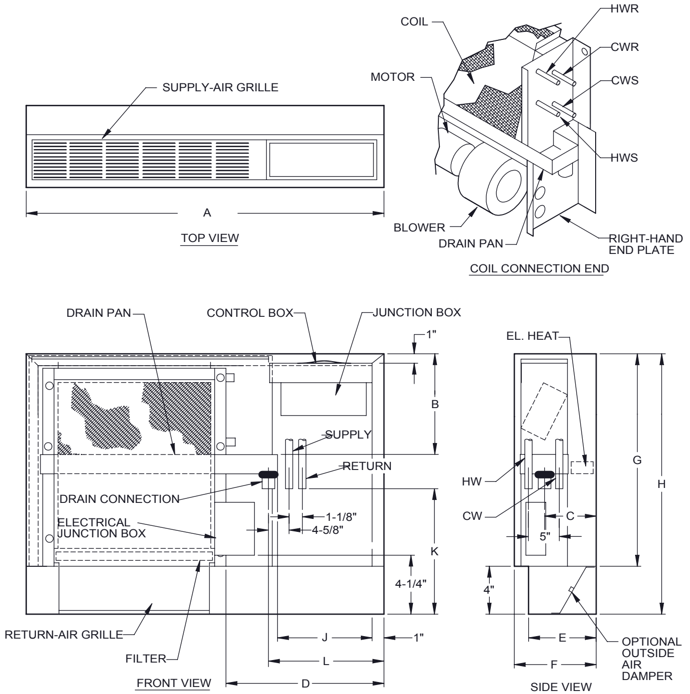
6" HANDED & 6" OPPOSITE CABINET EXTENSION & EXTENDED DRAIN PAN
