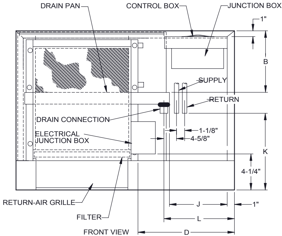
10" HANDED & 6" OPPOSITE CABINET EXTENSION & EXTENDED DRAIN PAN
