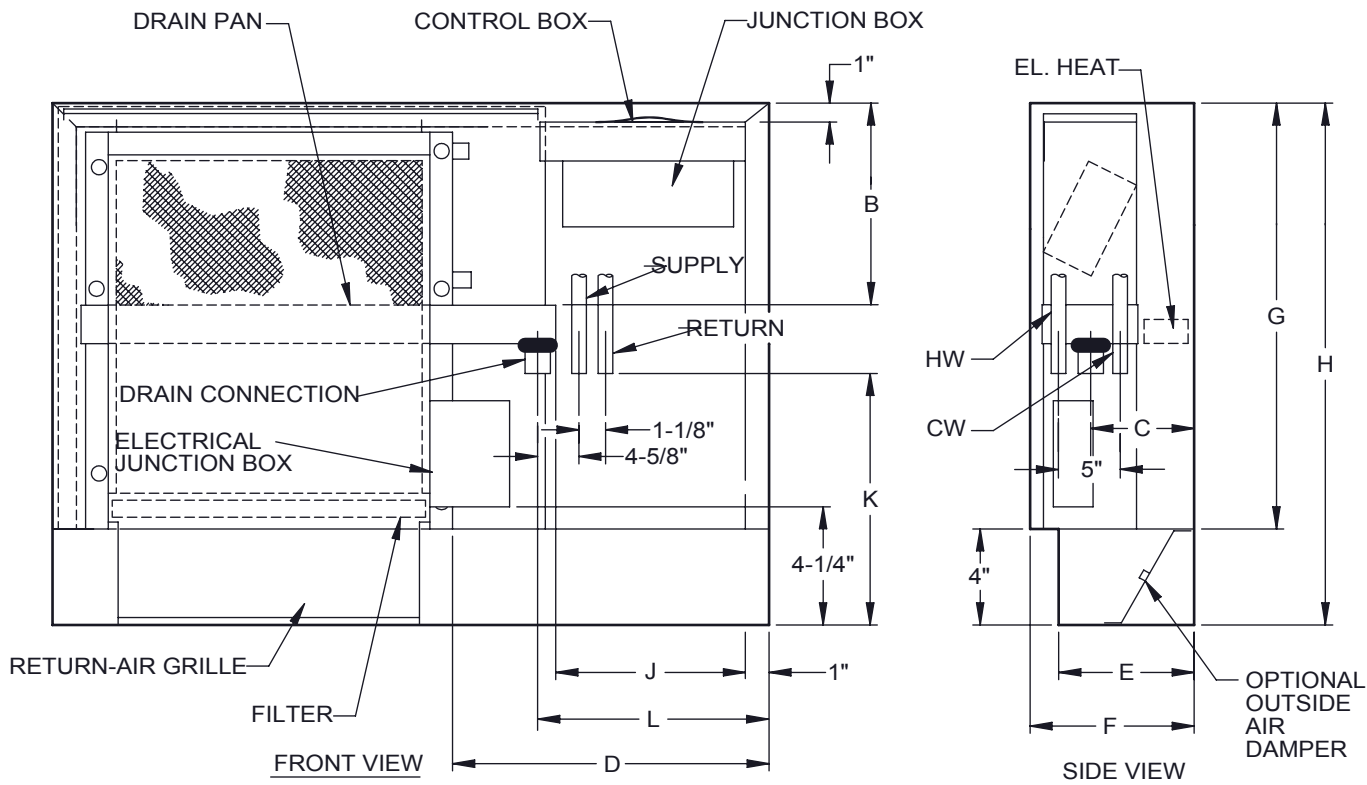
6" HANDED SIDE CABINET EXTENSION WITH EXTENDED DRAIN PAN
